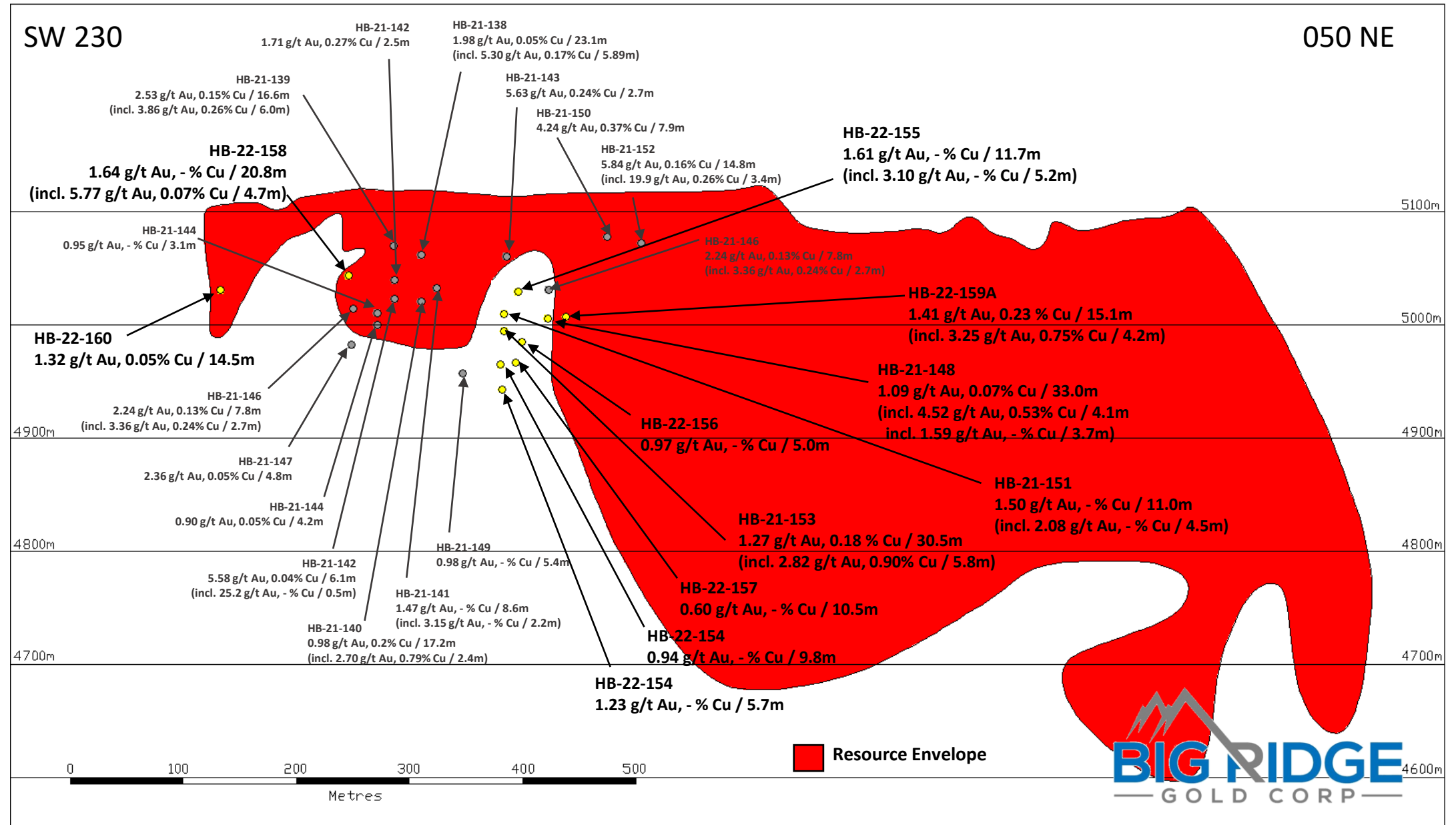
Figure 2: Longitudinal Section looking NW
